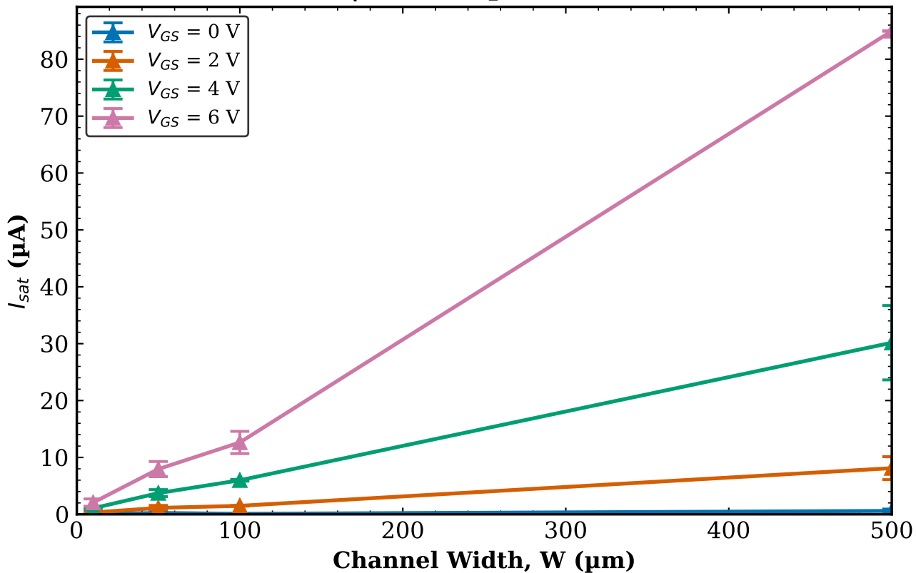
All Chips - Combined I_{sat} vs W | L = 80\text{ }\mu\text{m} (mean \pm std)
